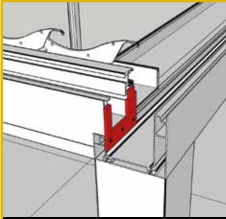
TEKLİ RAY ÖN LAZER MONTAJ DETAYI SINGLE RAIL FRONT LASER MOUNTING DETAIL
