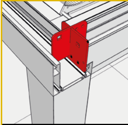
TEKLİ RAY ARKA LAZER MONTAJ DETAYI SINGLE RAIL REAR LASER MOUNTING DETAIL
