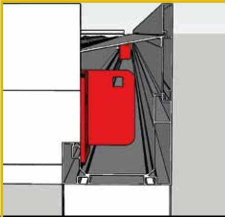
MOTOR LAZERİ MONTAJ DETAYI MOTOR LASER ASSEMBLY DETAIL
