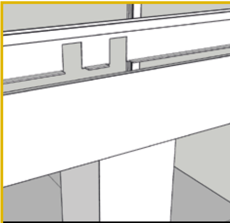
MOTOR KAPAĞI ÇİFTLİ RAY KERTME DETAYI ENGINE COVER DOUBLE RAIL NOTCH DETAIL
