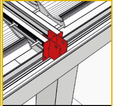
ÇİFTLİ RAY ARKA LAZER MONTAJ DETAYI DOUBLE RAIL REAR LASER MOUNTING DETAIL
