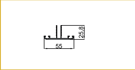
10-10091 Polikarbon Kapama Çıtasa Profili Polycarbonate Cover Strip Profile 0.252 kg/m
