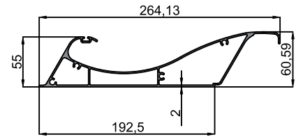
10-10944 Panel Profili / Panel Profile 3.490 kg/m
