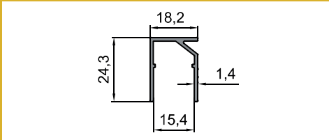
10-10095 Ayak Profili / Counterfort Profile 2.046 kg/m
