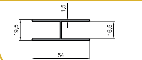
10-10090 H Profil / H Profile 0.505 kg/m
