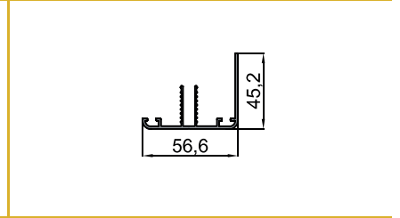
10-10559 Polikarbon Kapama Çıtasa Profili Polycarbonate Cover Strip Profile 0.210 kg/m
