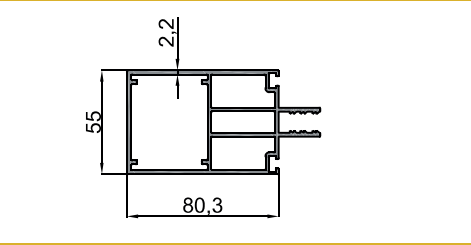
10-10101 Kutu Profil / Rectangular Tube Profile 1.582 kg/m
