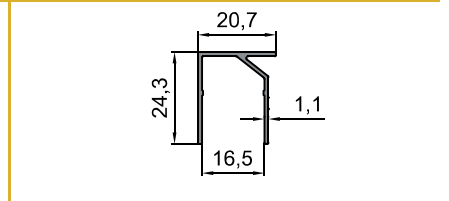
10-10096 Ayak Kapak Profili Counterfort Cover Profile 1.220 kg/m
