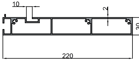
10-10943 Sabit Ray Profili / Stable Rail Profile 4.578 kg/m
