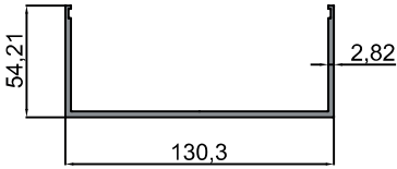
10-10545 Statik Profili / Static Profile 7.409 kg/m
