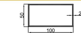
10-10101 Kutu Profil / Rectangular Tube Profile 1.582 kg/m
