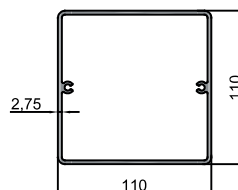
10-10103 Ayak Profili / Counterfort Profile 3.352 kg/m
