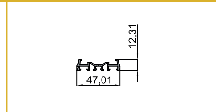
10-10453 Ayak Profili / Counterfort Profile 3.117 kg/m
