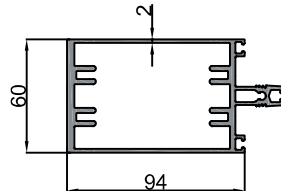
10-10103 Ayak Profili / Counterfort Profile 3.352 kg/m
