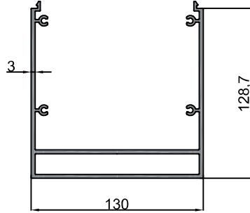
10-10560 Ayak Kapak Profili Kısa L Counterfort Cover Profile Short L 1.312 kg/m
