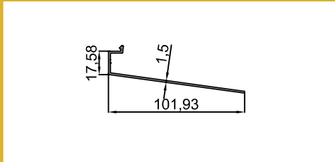
10-10456 Cam Tutucu Orta Kapak Profili Glazing Stop Middle Cover Profile 0.290 kg/m
