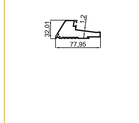
10-10452 Cam Tutucu Profil / Glazing Stop Profile 0.436 kg/m
