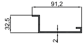
10-10942 Ayak Profili / Counterfort Profile 3.841 kg/m
