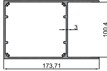
10-10291 Duvar Destek Profili Wall Back Up Profile 4.998 kg/m
