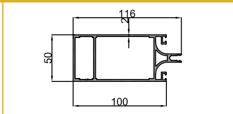
10-10457 Cam Tutucu Yan Kapak Profili Glazing Stop Side Cover Profile 0.436 kg/m
