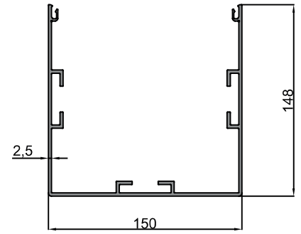
10-10944 Panel Profili / Panel Profile 3.490 kg/m
