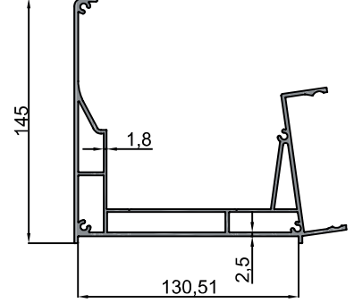
10-10528 Duvar Profili L / Wall Profile L 2.252 kg/m
