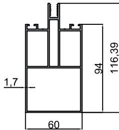
10-10554 Ayak Profili / Counterfort Profile 3.076 kg/m
