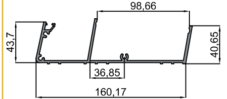
10-10528 Duvar Profili L / Wall Profile L 2.252 kg/m
