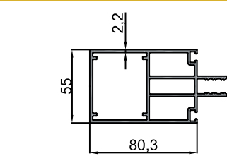
10-10101 Kutu Profil / Rectangular Tube Profile 1.582 kg/m
