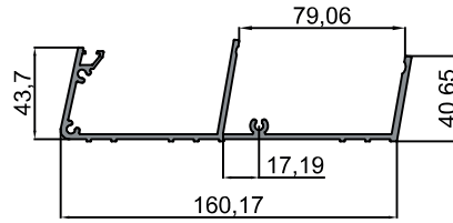
10-10537 Duvar Profili E / Wall Profile E 2.250 kg/m
