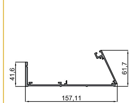
10-10093 Duvar Profili / Wall Profile 1.942 kg/m
