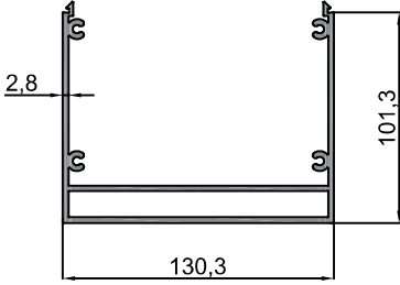
10-10538 Ayak Kapak Profili Uzun L Counterfort Cover Profile Long L 1.741 kg/m
