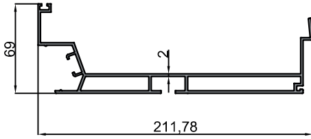
10-10974 Hareketli Ray Profili / Moving Rail Profile 1.493 kg/m
