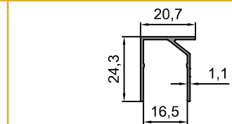
10-10096 Ayak Kapak Profili Counterfort Cover Profile 1.220 kg/m
