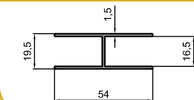
10-10090 H Profil / H Profile 0.505 kg/m
