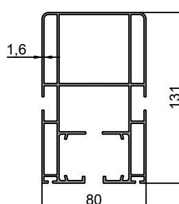
10-10541 80x130 mm Ray Profili/ 80x130 mm Rail Profile 3.613 kg/m
