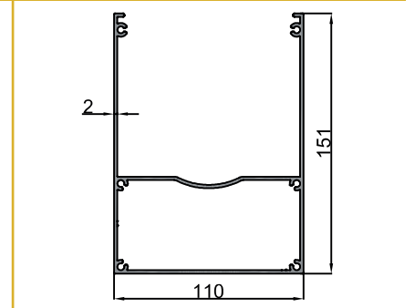
10-10453 Ayak Profili / Counterfort Profile 3.117 kg/m
