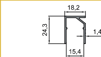
10-10095 Ayak Profili / Counterfort Profile 2.046 kg/m
