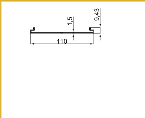
10-10449 Ayak Kapak Profili Counterfort Cover Profile 0.563 kg/m
