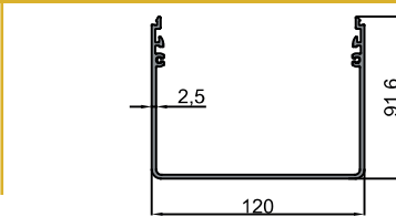
10-10095 Ayak Profili / Counterfort Profile 2.046 kg/m
