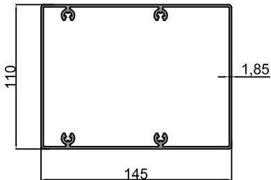
10-10554 Ayak Profili / Counterfort Profile 3.076 kg/m
