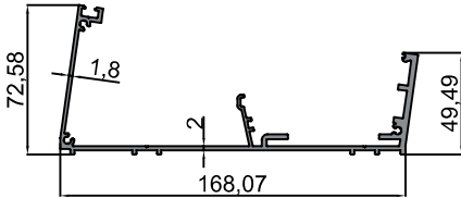
10-10553 Duvar Profili / Wall Profile 2.258 kg/m
