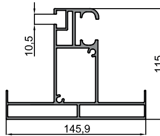
10-10943 Sabit Ray Profili / Stable Rail Profile 4.578 kg/m
