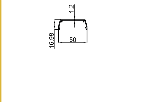
10-10449 Ayak Kapak Profili Counterfort Cover Profile 0.563 kg/m
