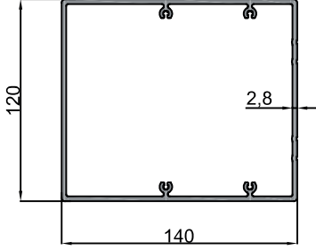
10-10283 Ayak Profili / Counterfort Profile 4.237 kg/m
