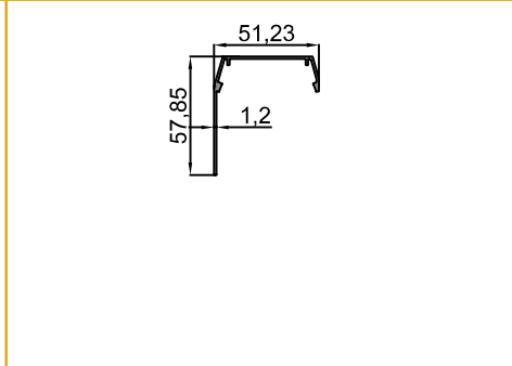
10-10457 Cam Tutucu Yan Kapak Profili Glazing Stop Side Cover Profile 0.436 kg/m
