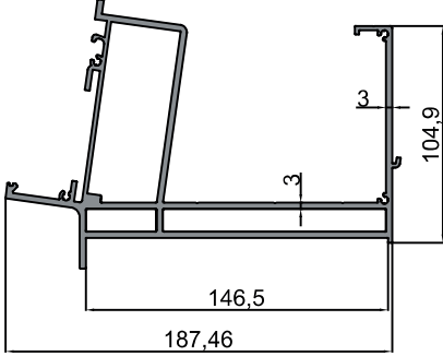
10-10553 Duvar Profili / Wall Profile 2.258 kg/m
