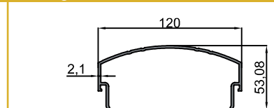
10-10096 Ayak Kapak Profili Counterfort Cover Profile 1.220 kg/m
